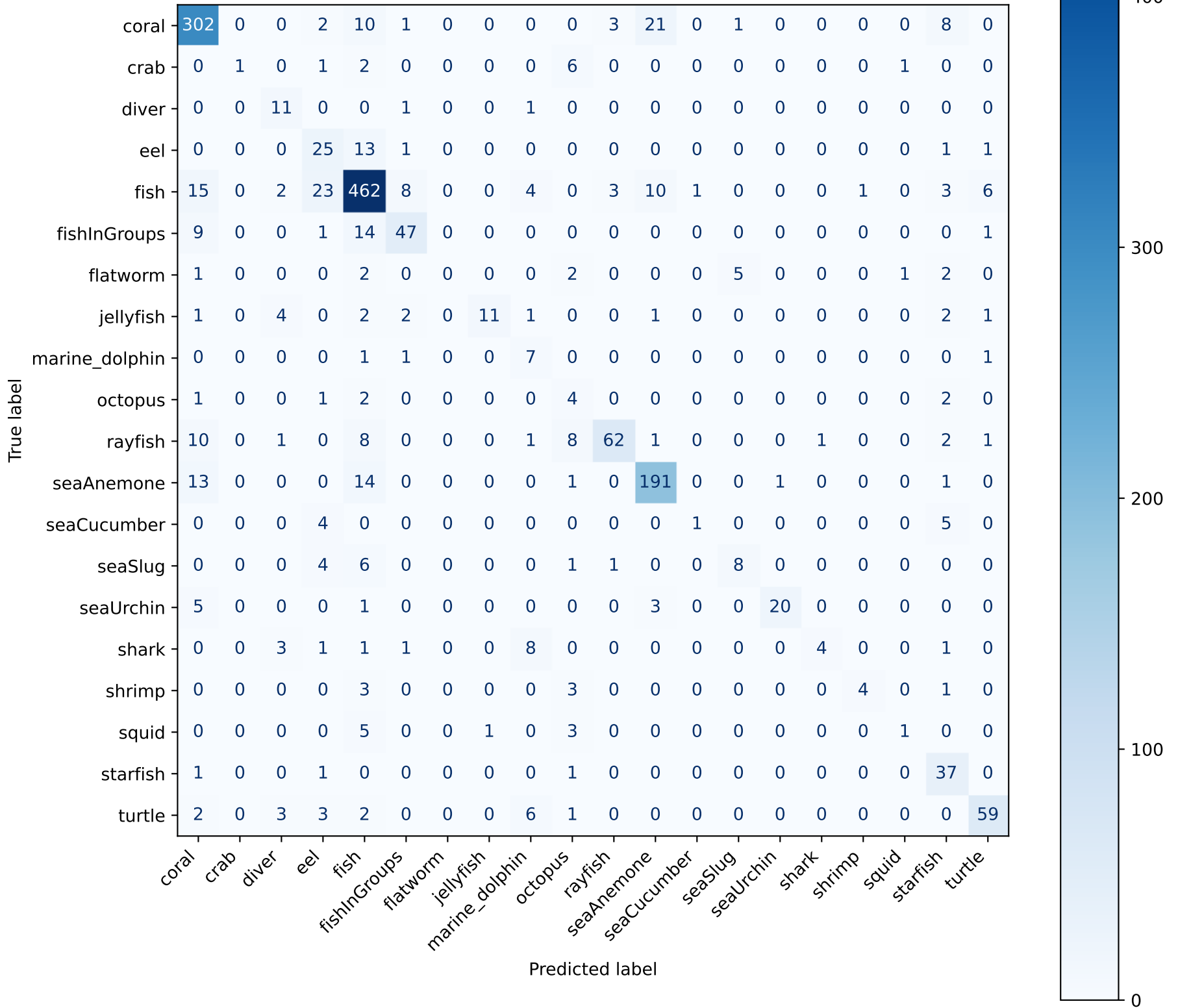
Confusion Matrix for vgg19
