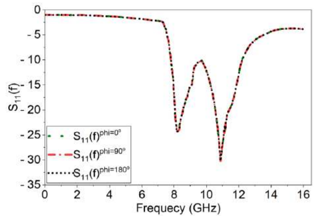
FIGURE 14: Reflectance measurement with variation in polarization angle ( \phi ).
