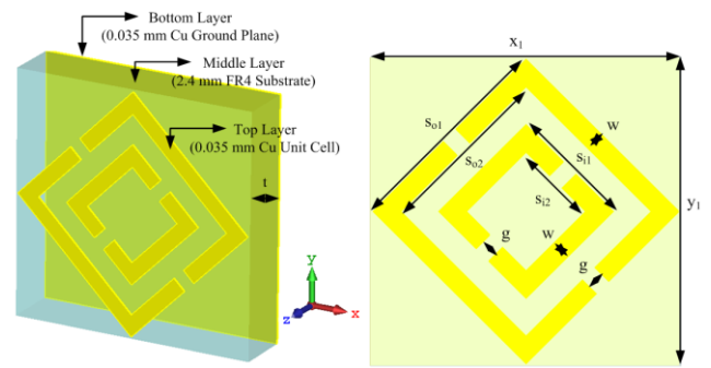
FIGURE 1. Dimensional structure of DBSSRMMA unit cell.
