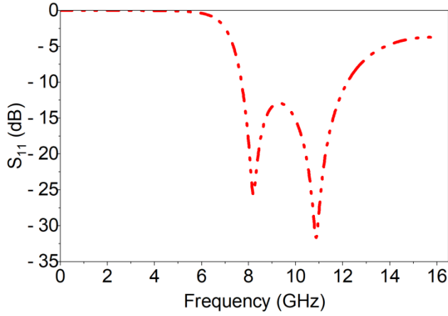
FIGURE 6: Reflectance S_{11}(f) of the DBSSRMMMA structure.
