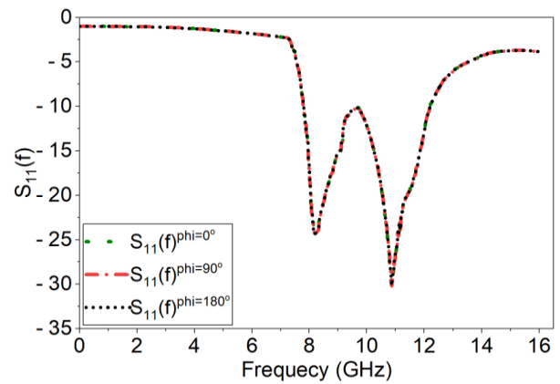
FIGURE 14: Reflectance measurement with variation in polarization angle ( \varphi ).
