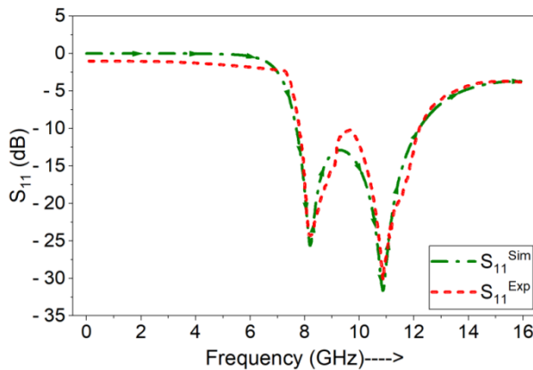
FIGURE 13: Comparison of simulated and measured reflectance.
