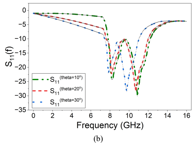
FIGURE 15: Reflectance measurement with variation in incidence angle ( \theta ).
