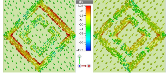
FIGURE 8: Surface current distribution at (a) 8.2 GHz. (b) 10.87 GHz.
