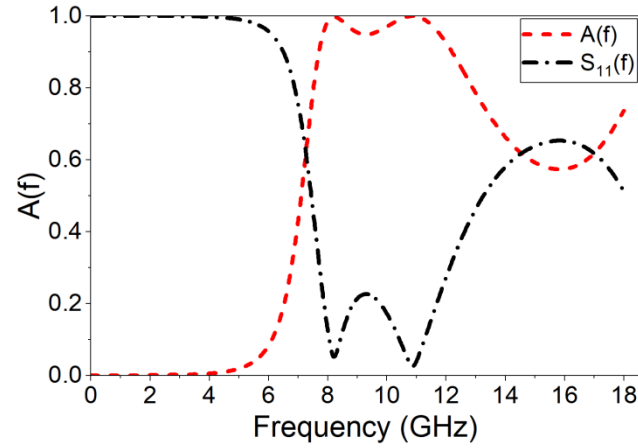
FIGURE 7: Linear Absorbance A(f) and Reflectance S_{11}(f) .
