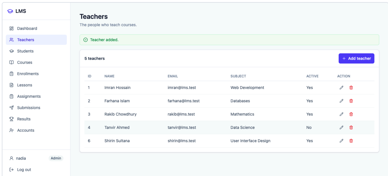
Figure 8.1 The green "Teacher added." banner after a save. The screenshot was taken before the banner gained its close button, so it sits full width and without the ×.
