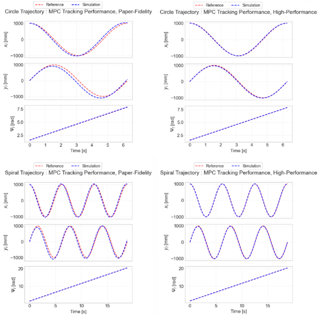
Figure 7. The temporal evolution of the inertial states for the Circle and Spiral trajectories. The 2x2 grid compares the Paper-Fidelity strategy (left) against the High-Performance configuration (right).
