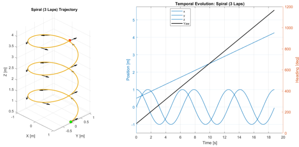
Figure 2. Visualization of the spiral trajectory: (a) Spiral Trajectory in 3D space. (b) Evolution of x , y , z , and \Psi during T_{\text{spiral}} .
