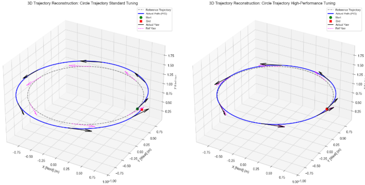
Figure 8. Circle Trajectory Results for PID.
