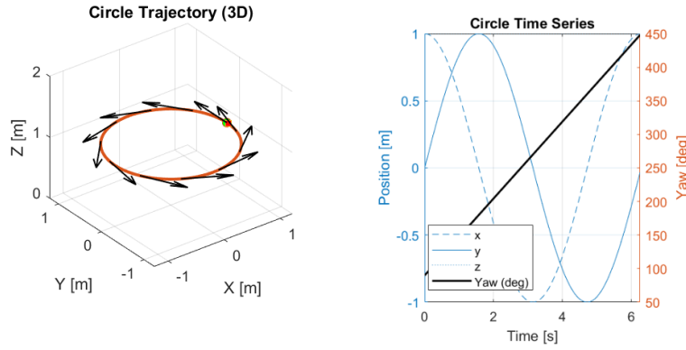
Figure 1. Visualization of the circle trajectory with the tangent yaw mode: (a) Circle Trajectory in 3D space. (b) Evolution of x , y , z , and \Psi during T_{\text{circle}} .
