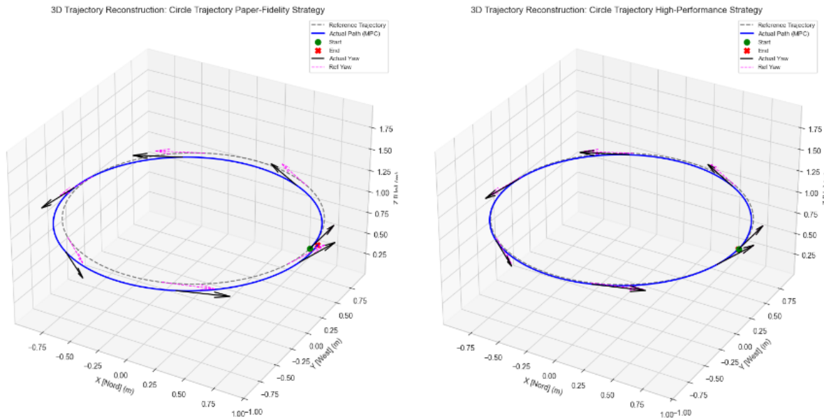
Figure 5. Circle Trajectory Results for MPC.
