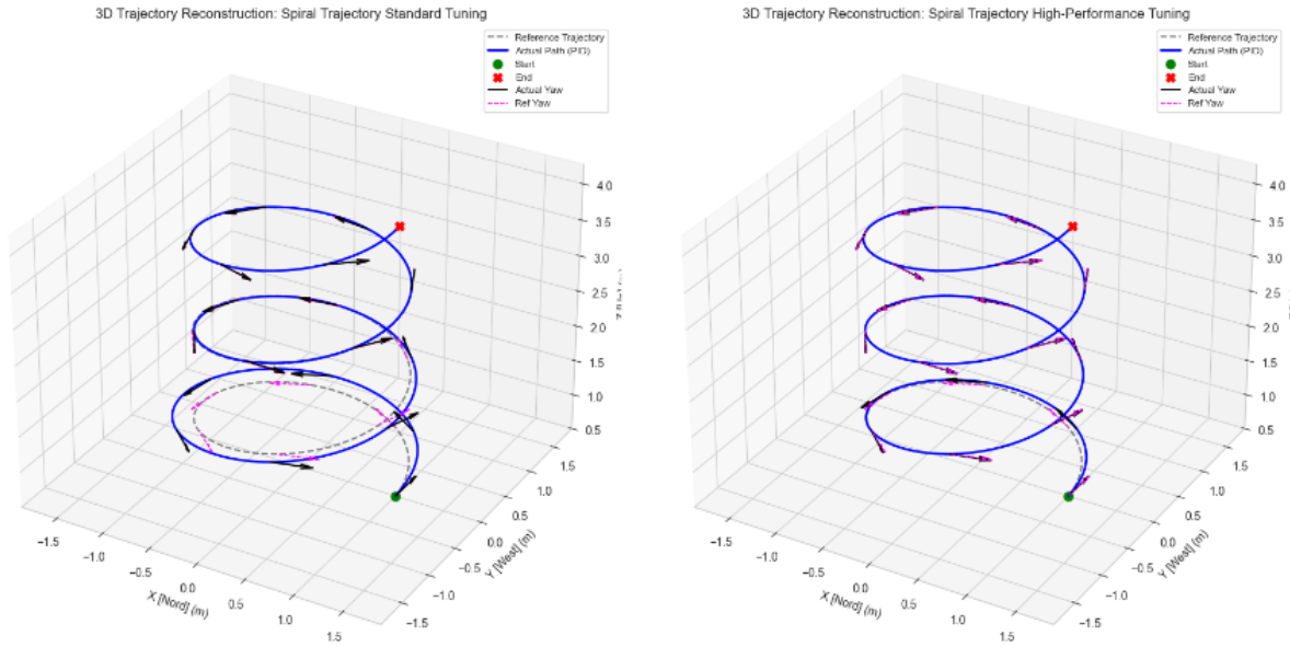
Figure 9. Spiral Trajectory Results for PID.
