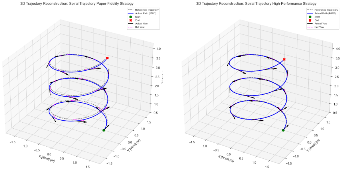
Figure 6. Spiral Trajectory Results for MPC.
