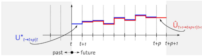
Figure 4. Visualization of the warm-start strategy: the previous optimal control sequence is shifted forward to provide a consistent nominal trajectory for the next LTV linearization.
