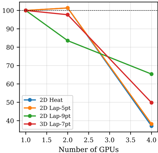
Scaling Efficiency
