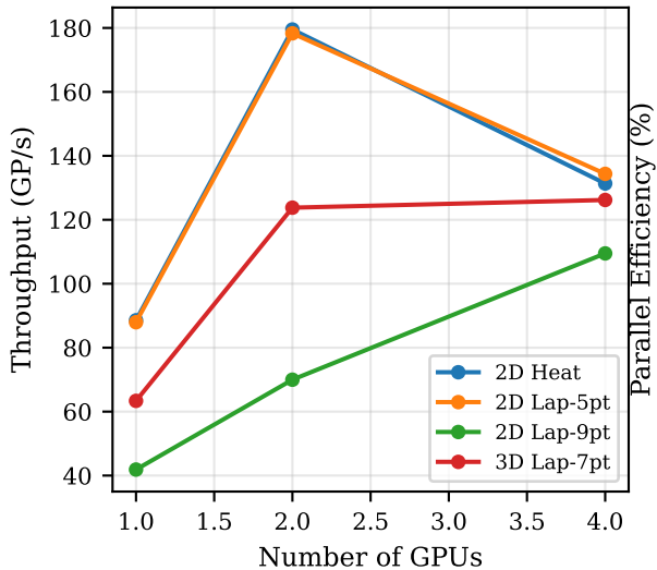
Strong Scaling
