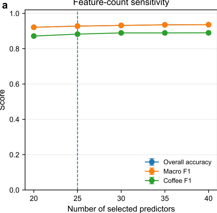
Feature-count sensitivity
