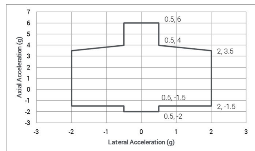
Figure 5: Payload maximum design load factors
