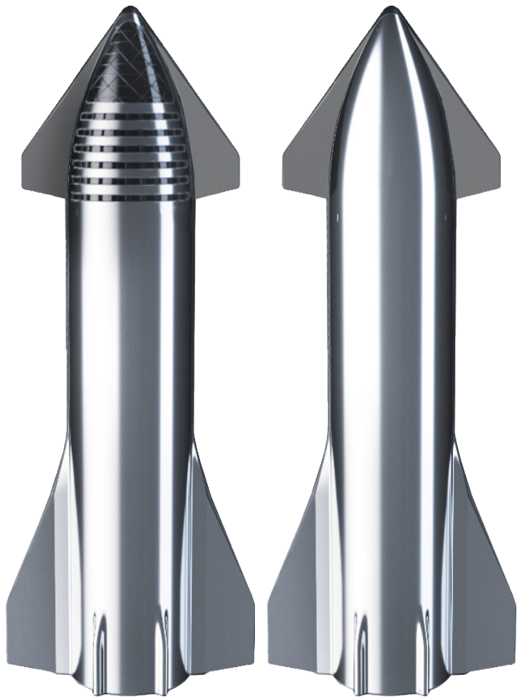
Figure 2: Starship crew (left) and uncrewed (right) configurations
