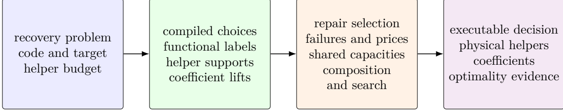
Figure 2: Ergodis separates the source model, admitted representation, optimization, and evidence contract. Functional labels preserve composition; support alternatives preserve overlap and helper-price queries. Stored lifts reconstruct feasible decisions, while optimality needs a matching checked bound or complete search justification. Reuse under updates or new readouts requires admission for the chosen observation. The mathematical results do not depend on executing this pipeline.
