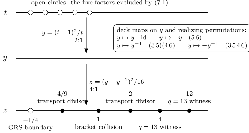
Figure 2: The degree-eight quotient of the admitted pencil (special points on the z -line are arranged schematically). The parameter t double-covers y = (t - 1)^2/t , and the four identifications y \mapsto \pm y^{\pm 1} , each realized by a displayed party permutation, cover z . The open point z = -1/4 is the excluded GRS boundary; z = 1 is a bracket collision; z = 4, 12 form the q = 13 four-copy witness pair; and z = 2, 4/9 belong only to the transport-rank detector, not to the LU-orbit boundary.
