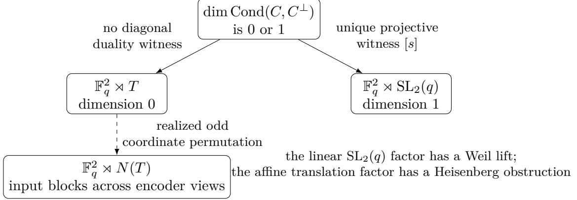
Figure 1: The dimension of the code-to-dual conductor selects the exact fixed-coordinate projective transversal group. Coordinate permutations form a separate extension problem: in the computed non-GRS rows, an odd permutation enlarges the possible input blocks from T to N(T) across encoder views, but it need not fix the chosen encoder input.
