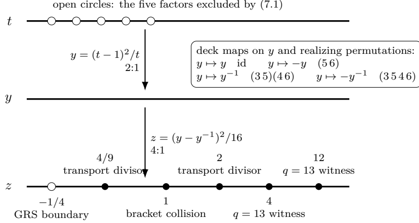
Figure 6: The degree-eight quotient of the admitted pencil (special points on the z -line are arranged schematically). The parameter t double-covers y = (t-1)^2/t , and the four identifications y \mapsto \pm y^{\pm 1} , each realized by a displayed party permutation, cover z . The open point z = -1/4 is the excluded GRS boundary; z = 1 is a bracket collision; z = 4, 12 form the q = 13 four-copy witness pair; and z = 2, 4/9 belong only to the transport-rank detector, not to the LU-orbit boundary.
