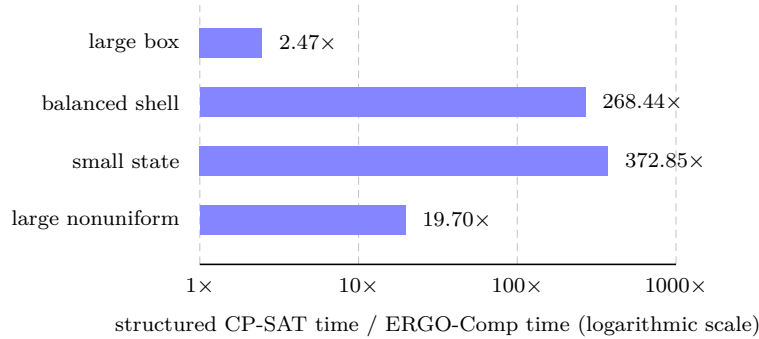
Figure 2: ERGO-Comp speedup over structured CP-SAT on the four recorded exact scheduler profiles. Both solvers receive the same safe preprocessing and must return the same optimum and retained loads. The bars summarize the exact medians in Table 1; they are bounded implementation measurements, not a general solver ranking.
