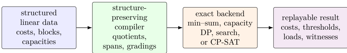
Figure 1: ERGO-Comp turns proved structural reductions into exact optimization. The compiler preserves enough labels to reconstruct a coefficient-level witness; it may solve the reduced state space directly or leave general side constraints to CP-SAT. The mathematical results do not depend on executing this pipeline.
