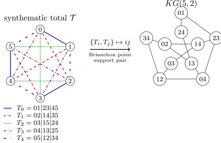
Figure 1: The synthemetic–Petersen dictionary. The five self-polar triangles give the displayed perfect matchings. A Petersen vertex ij represents the Brianchon point and complementary support pair attached to \{T_i, T_j\} ; two vertices are adjacent when the index pairs are disjoint.
