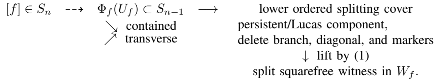
Fig. 1. Coherent polar induction. The contained branch is a level-specific component theorem; only the transverse branch is controlled by the general point-count argument.
