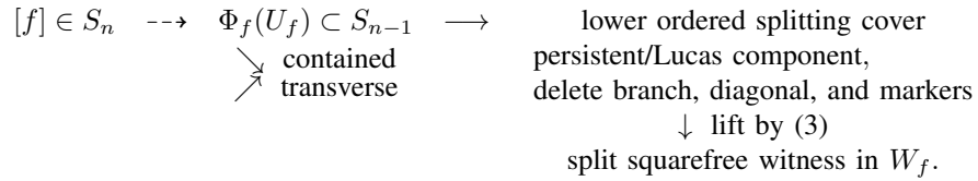
Fig. 1. Coherent polar induction. The contained branch is a level-specific component theorem; only the transverse branch is controlled by the general point-count argument.
