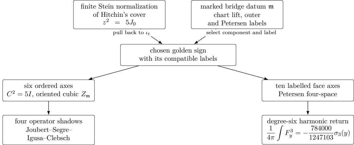
Figure 2: The source–shadow–return scheme. Solid arrows are constructions after the two top inputs have been fixed. The lower branches compare the chosen sign; they neither identify the displayed cubics nor define a map between their ambient harmonic spaces.
