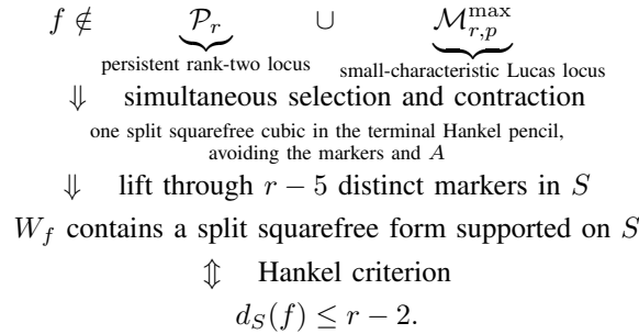
Fig. 1. The proof route. The carrier theorem identifies the only possible obstruction; simultaneous contraction constructs a locator everywhere else.
