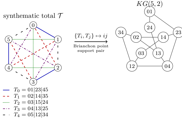
Figure 2: The synthematic–Petersen dictionary. The five line styles encode the five self-polar triangles as perfect matchings of the six coordinates. For each pair \{T_i, T_j\} , their union is an alternating six-cycle: its opposite-edge matching gives a Brianchon point, and its alternating vertex classes give a complementary support pair. Both are represented by the Petersen vertex ij ; adjacency means that the index pairs are disjoint.
