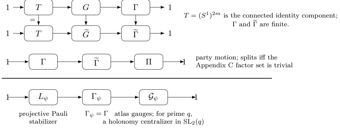
Figure 4: The layered symmetry group of a stabilizer AME state. One-site phases form the identity component, with finite fixed-party and party-moving projective quotients. The fixed-party quotient is itself an extension of the atlas gauge group by the projective Pauli stabilizer. Independently, allowing party motion extends the fixed-party projective group by the realized permutation group, with splitting governed by a nonabelian factor set.
