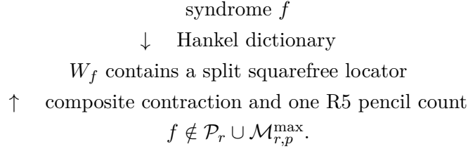
Figure 1: The proof route. The carrier theorem identifies the only possible obstruction; simultaneous contraction constructs a locator everywhere else.
