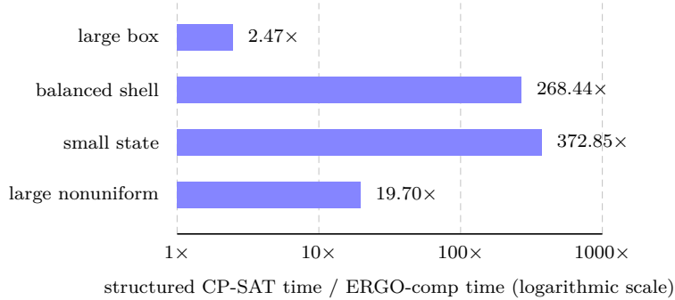
Figure 3: ERGO-comp speedup over structured CP-SAT on the four recorded exact scheduler profiles. Both solvers receive the same safe preprocessing and must return the same optimum and retained loads. The bars summarize the exact medians in Table 1; they are bounded implementation measurements, not a general solver ranking.
