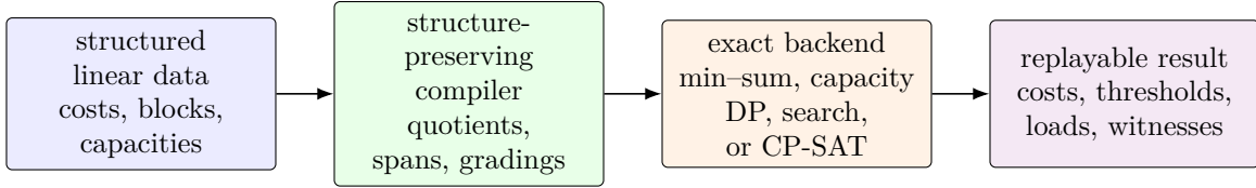
Figure 2: ERGO-comp turns proved structural reductions into exact optimization. The compiler preserves enough labels to reconstruct a coefficient-level witness; it may solve the reduced state space directly or leave general side constraints to CP-SAT. The mathematical results do not depend on executing this pipeline.
