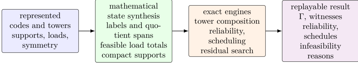
Figure 2: ergodis synthesizes the exact state exposed by the mathematics before search begins. Labelled coset costs drive tower composition, support families drive reliability, and feasible load totals are the states used in scheduling. Large support families may be stored by a zero-suppressed decision diagram (ZDD), which shares repeated choices. For attained fibres, stored lifts expand an optimum to a coefficient-level witness or obstruction; supported residual side constraints may be passed to CP-SAT. The mathematical results do not depend on executing this pipeline.
