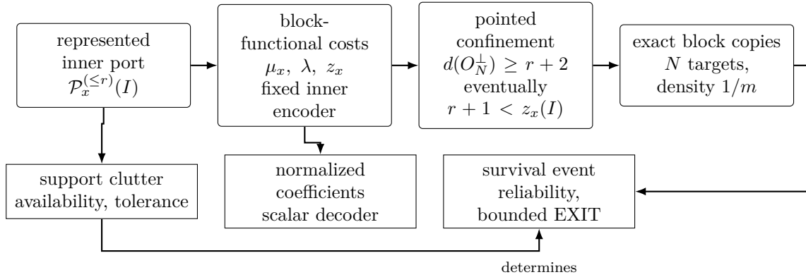
Figure 1: The transfer spine. In the fixed-inner, L -linear concatenation regime, weighted block-functional costs give an exact confinement gate. When d(O_N^\perp) \rightarrow \infty and r + 1 < z_x(I) , support and normalized coefficient ports are copied into every block. Reliability is derived from the copied support clutter; the diagram makes no necessity claim for arbitrary asymptotically good families.
