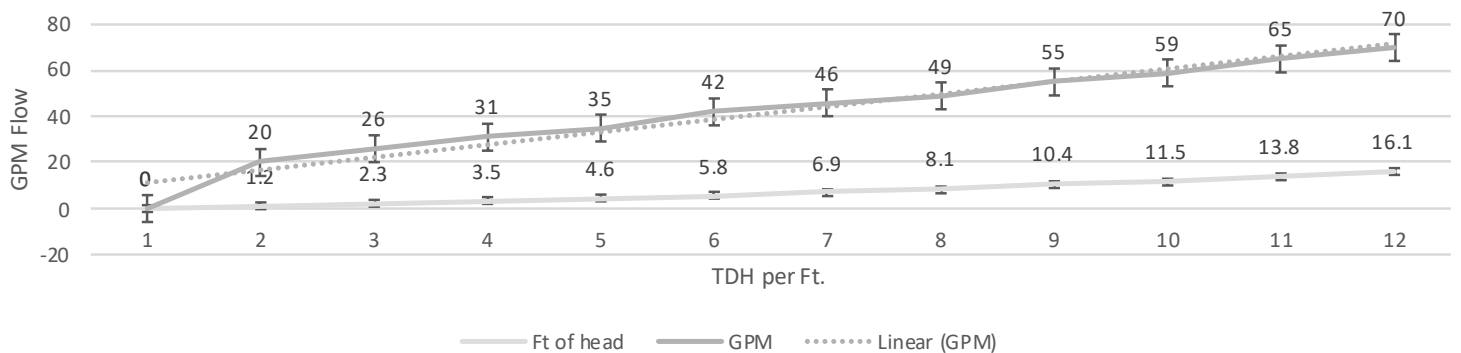
Head Loss
