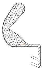
12652 reach .730"
