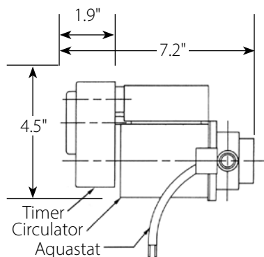
Assembled Timer/Aquastat
