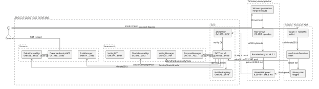
Fig. 4. ZK-PZ Protocol Architecture: off-chain proving pipeline and on-chain settlement
