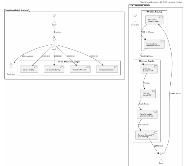
Fig. 2. Traditional Zakat Paradigm vs. Proposed ZK-PZ Model
