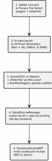
Fig. 5. ZK-PZ Donation Flow: from wallet connection to SBT receipt to the donor
