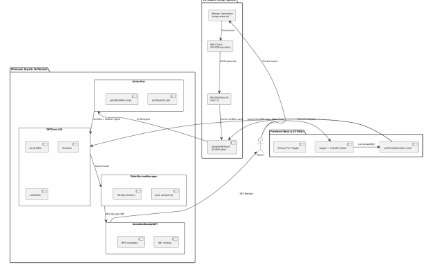
Fig. 4. ZK-PZ Protocol Architecture: off-chain proving pipeline and on-chain settlement
