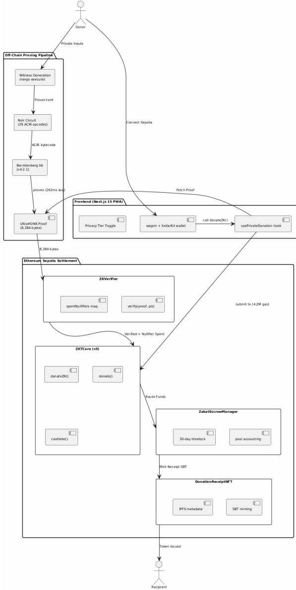
Fig. 4. ZK-PZ Protocol Architecture: off-chain proving pipeline and on-chain settlement
