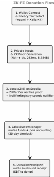
Fig. 5. ZK-PZ Donation Flow: from wallet connection to SBT receipt to the donor
