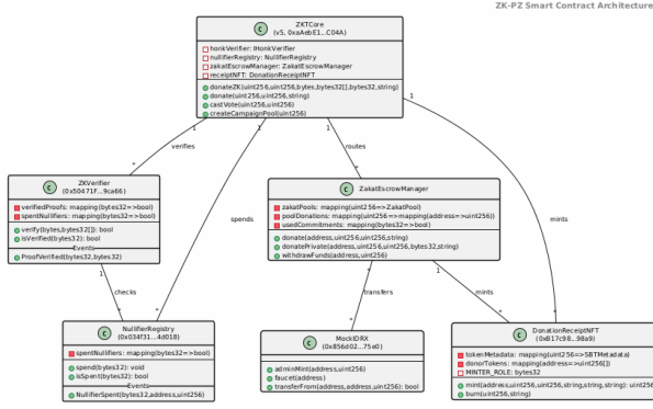
Fig. 6. ZK-PZ Smart Contract Architecture with Sepolia addresses and cardinality
