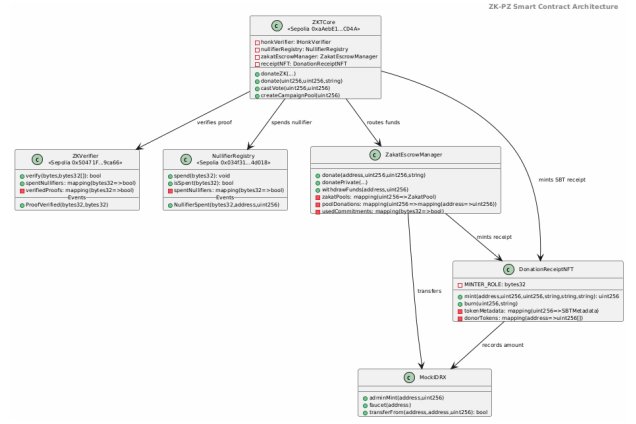
Fig. 5. ZK-PZ Smart Contract Architecture with Sepolia addresses
