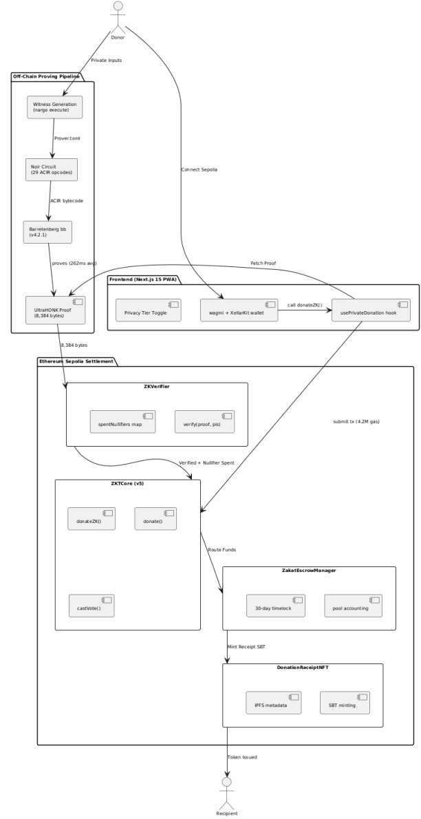
Fig. 3. ZK-PZ Protocol Architecture: off-chain proving pipeline and on-chain settlement
