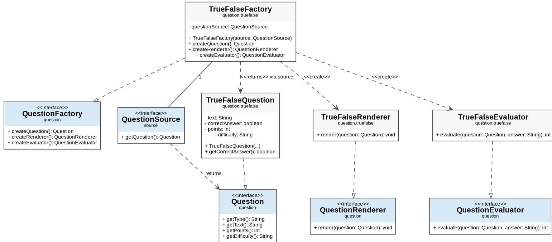
Figure 4. Abstract Factory Pattern - True/False Product Family
