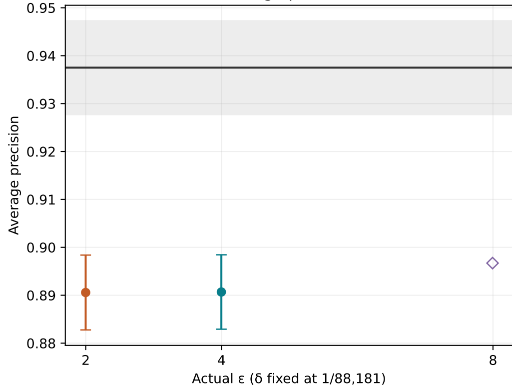
Average precision
