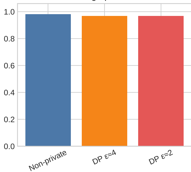
Average precision
