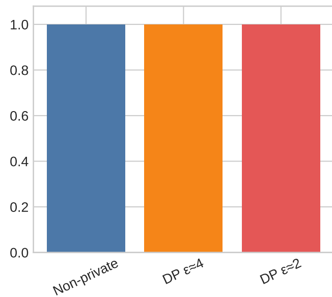
Recall
