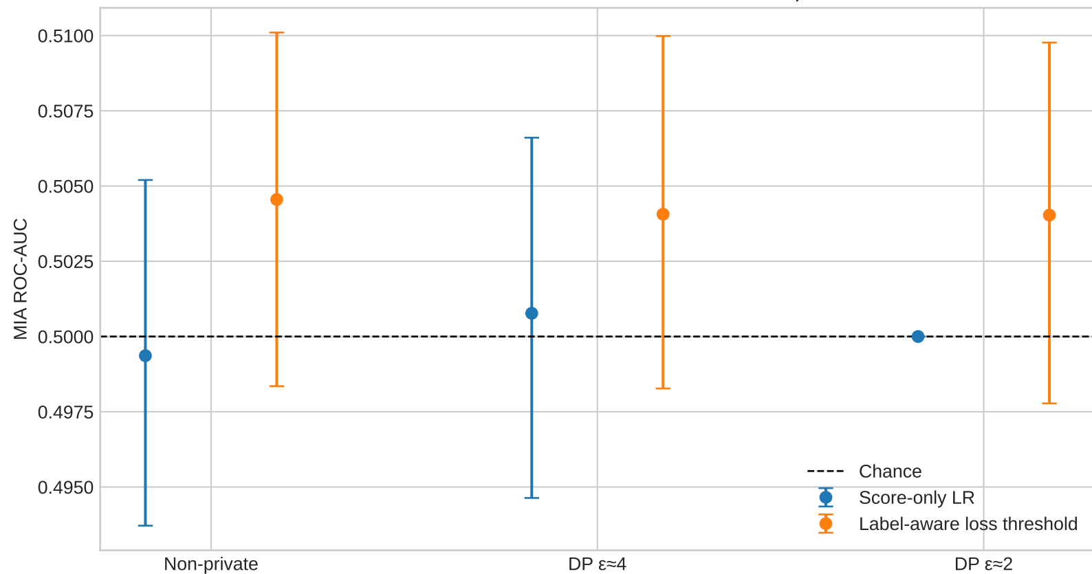
UNSW-NB15 MIA AUC with 95% stratified bootstrap intervals
