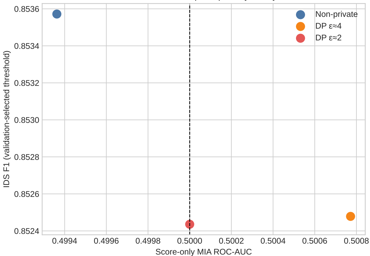
UNSW-NB15 descriptive privacy–utility view
