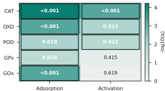
A BH q values | 8/10 retained
