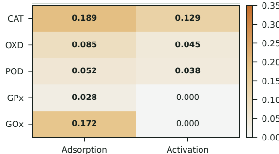
B Epsilon-squared effect size
