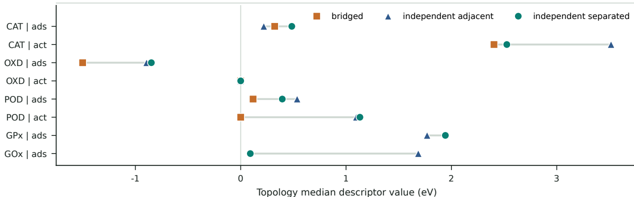
C Topology medians for retained activity-descriptor pairs
