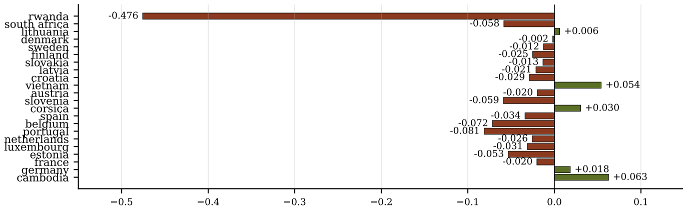
\Delta \text{Pixel IoU} (Planet B3 augmax full – S2 PRUE-B7 full)
