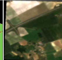
S2 (10 m)
