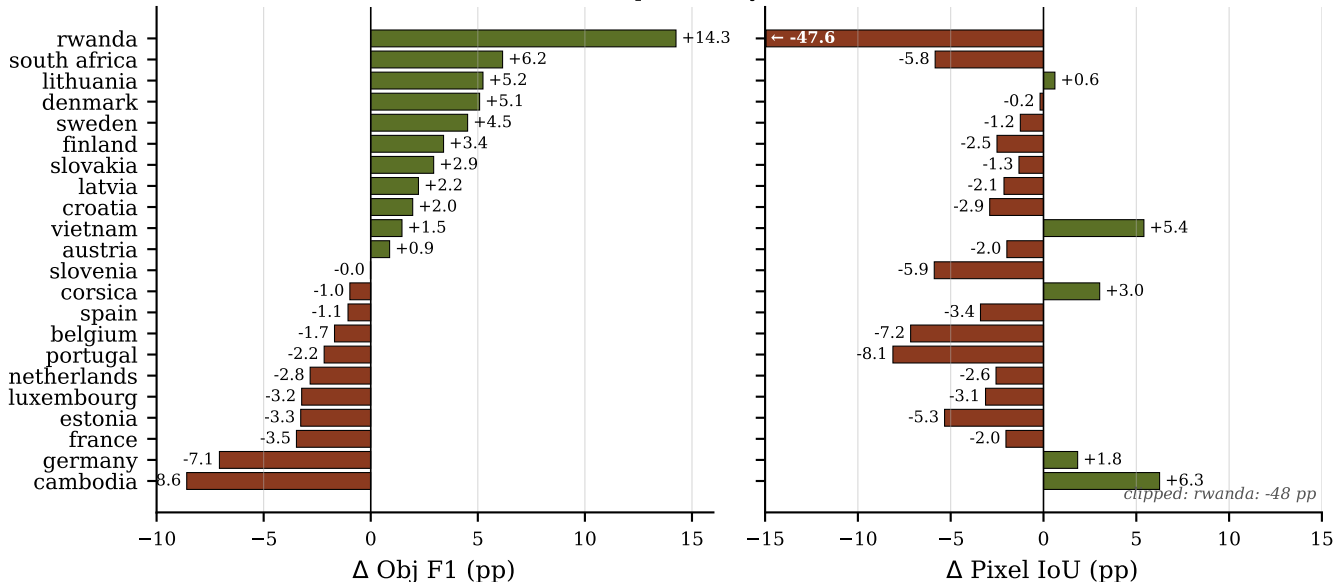
FTW-HD (3\,m) vs Sentinel-2 PRUE-B7 full (10\,m): per-country deltas (olive = Planet wins, sienna = S2 wins)
