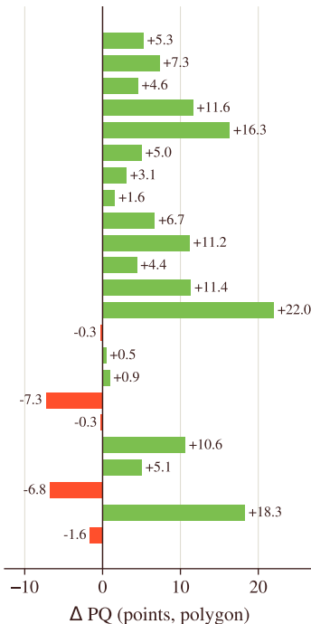
Polygon PQ
