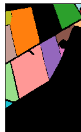
Watershed instances
