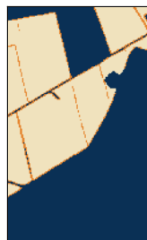
Prediction (3-class)
