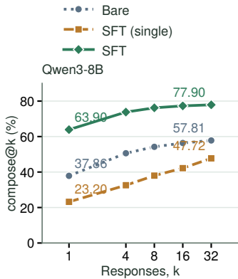
Figure 4: Effect of SFT label construction on Qwen3-8B compose@k.
