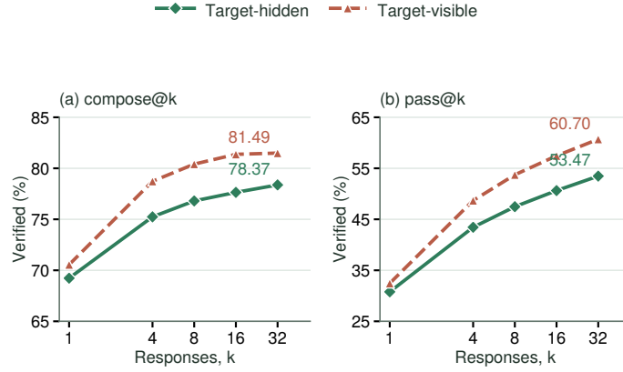
Figure 10: Target visibility for Qwen3-8B SFT+RL: (a) compose@ k ; (b) pass@ k .
