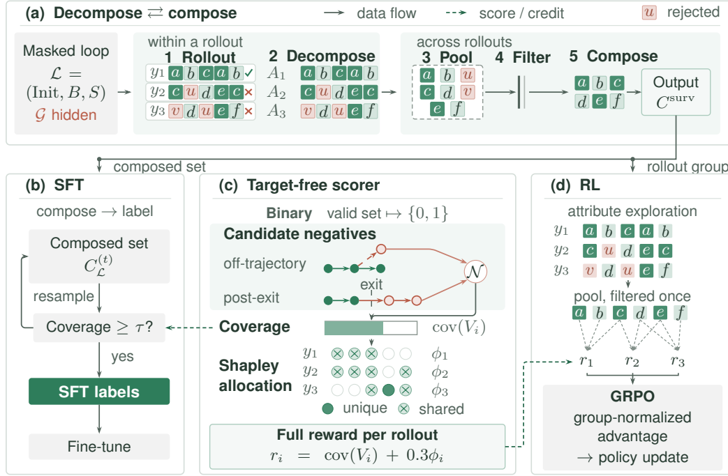
Figure 1: Decompose-compose is the organizing principle. (a) Pooling and joint filtering retain useful clauses from failed responses; letters track clause identity. (b) SFT distills coverage-accepted compositions. (c) Execution-derived candidate negatives supply coverage; Shapley allocation splits shared rejection credit. (d) Retained clauses credit their proposing rollouts for GRPO. The sampler inset shows off-trajectory perturbations and post-exit body continuations. The hidden target \mathcal{G} is restored only for final verification.
