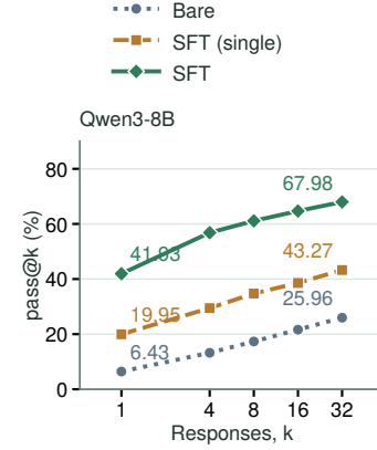
Figure 7: Effect of SFT label construction on Qwen3-8B pass@k.
