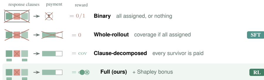
Figure 4: The four credit rules ablated in Section 4.6, applied to one shared rollout group with two valid clauses (green) and one malformed clause (red). Response-level gates (top two rows) void the whole payment: Binary pays a single \{0, 1\} token and Whole-rollout computes coverage but pays nothing unless every clause survives. Clause-level gates (bottom two rows) pay each surviving clause; Full adds the closed-form Shapley bonus for shared rejections (filled: unique, crossed: shared).
