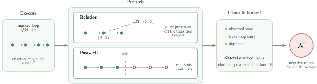
Figure 2: Construction of target-hidden negative traces. Concrete executions provide observed reachable states. Two transformations probe relational structure and behavior past a genuine exit. Conservative cleaning selects these traces first, then random perturbations fill the common 60-trace budget. The resulting \mathcal{N} is used for SFT acceptance and RL reward computation and never exposes Q .
