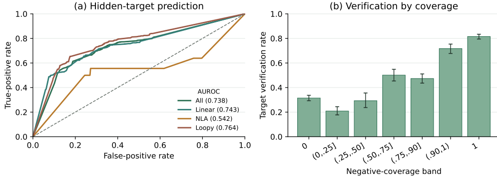
Figure 5: Predictive validity of target-independent negative coverage on saved test-set candidates. (a) ROC curves for restored-target verification; numbers in parentheses are AUROCs. (b) Target verification rate by coverage band, with Wilson 95% intervals. NLA remains close to chance, showing that the current structured negatives discriminate hidden-target utility much better for Linear and Loopy programs than for nonlinear arithmetic.
