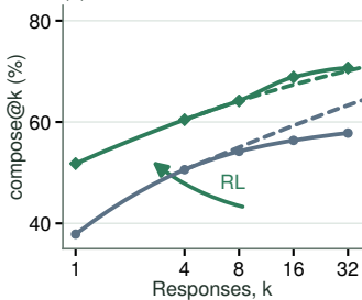
(a) Bare \rightarrow RL
