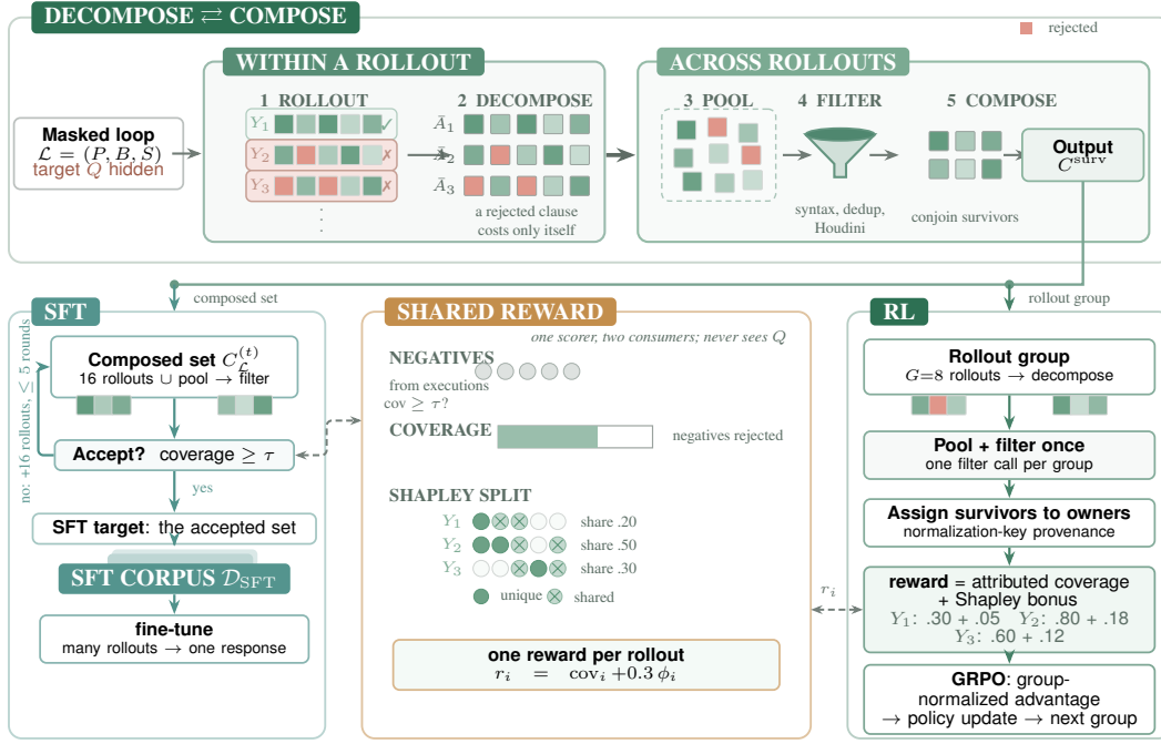
Figure 1: Decompose-compose is the organizing principle. Each target-hidden rollout is decomposed into clauses, and their union is composed into one filtered invariant (top). One target-independent reward (center) scores clause sets against execution-derived negatives and is shared by both training stages. Left: SFT accepts a composed set once its whole-rollout coverage of the negatives reaches \tau , strengthening it with further rollout groups otherwise, and distills each accepted set into one response. Center: the reward combines coverage of the negatives with a closed-form Shapley bonus for shared rejections, paying r_i = \text{cov}_i + 0.3 \phi_i per rollout; the alternative credit rules are evaluated in Section 5.6. Right: RL pools and filters each rollout group once, assigns survivors to owners by normalization-key provenance, combines attributed coverage and the Shapley bonus into one reward, and applies a GRPO update. The hidden target Q is restored only for the final proof of the composed output; neither generation nor training ever sees it.
