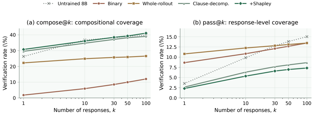
Figure 4: Reward-function ablation on Qwen3-8B (three-seed means). Binary and whole-rollout credit raise response-level accuracy at small budgets (b) but flatten compositional coverage (a). Clause decomposition reverses this trade-off, and Shapley credit shifts the compose curve further toward the upper left: both dominate the response-level variants at every k in (a), and Shapley credit also ends above the untrained model at k=32 (TBD vs. TBD). Exact numbers for all variants appear in Table 14 (Appendix I.4).
